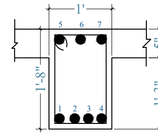
SECTION 1-1
