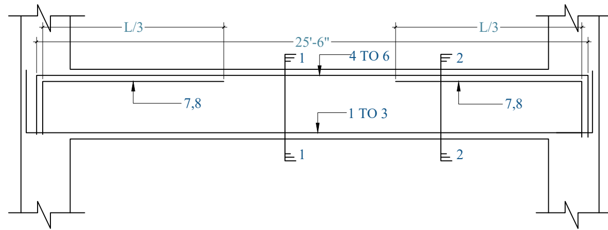
L-SECTION OF BEAM B-1
