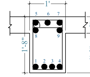
SECTION 2-2
